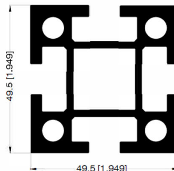
PERFIL 50mm X 50mm 32184
