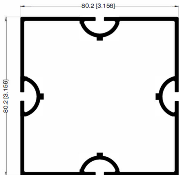
PERFIL 80mm X 80mm 30797
